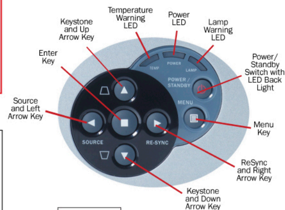
Control Panel
