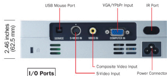
I/O Ports
